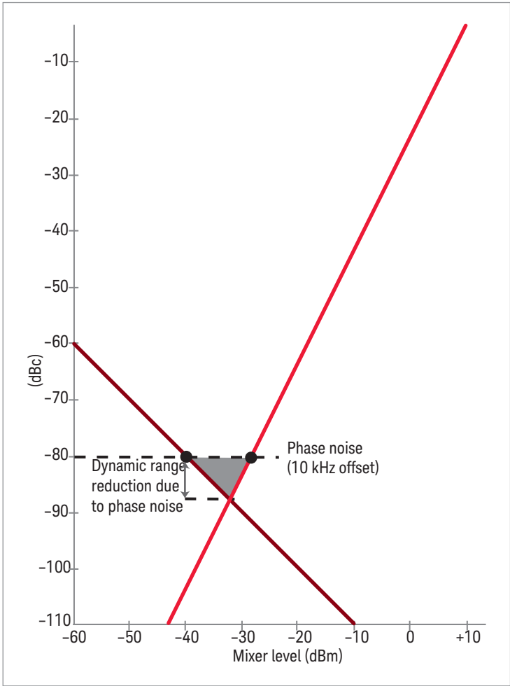
Figure 6-4. Phase noise can limit third-order intermodulation tests
