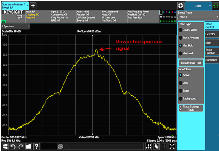
Figure 2-37. Frequency domain view of the GSM signal with 2 time slots “on” showing an unwanted spurious signal present in the spectrum.
