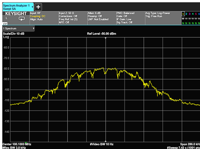
Figure 2-32a. Video filtering
