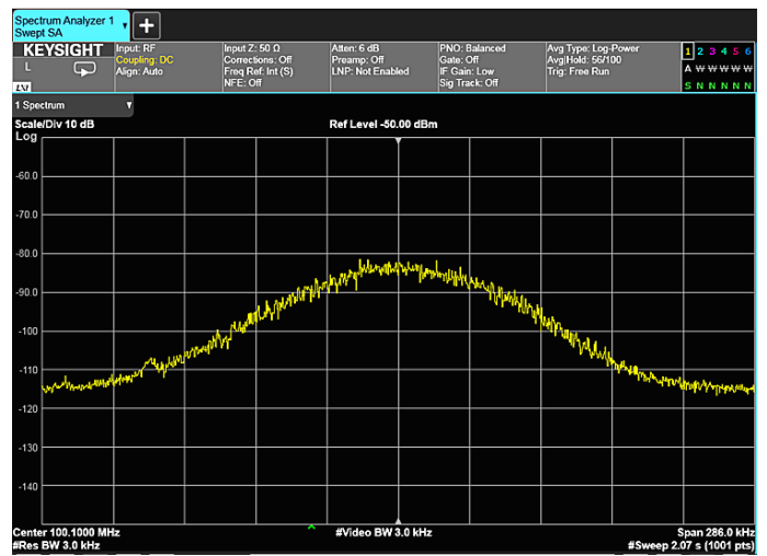
Figure 2-32b. Trace averaging
