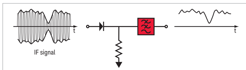
Figure 2-15. Envelope detector
