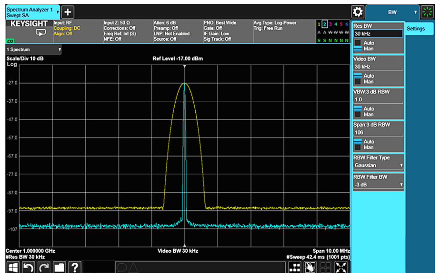
Figure 5-2. Displayed noise level changes as 10 \log (BW_2/BW_1)
