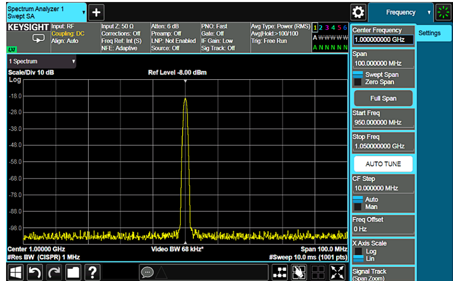
Figure 2-18. Each of the 1001 trace points (buckets) covers a 100-kHz frequency span and a 0.01-millisecond time span
