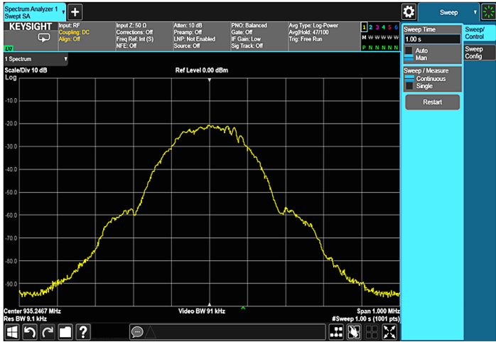
Figure 2-39. Spectrum of time slot 3 reveals that the spurious signal is not caused by this burst.
