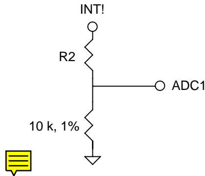
Figure 6-4. Schematic of the light sensor
