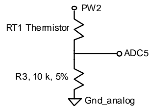
Figure 2-1. Thermistor Schematic
