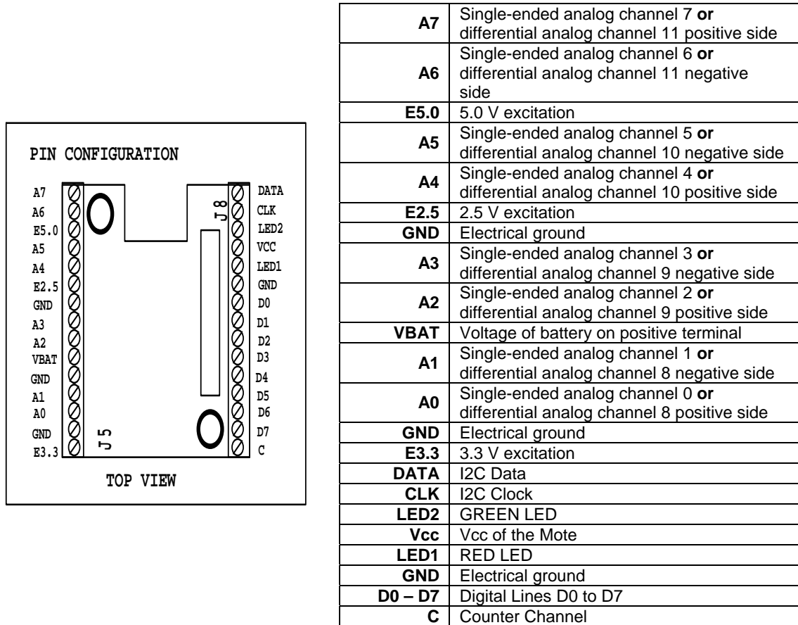
Figure 8-2. Pin configuration and assignments of the MDA300CA
