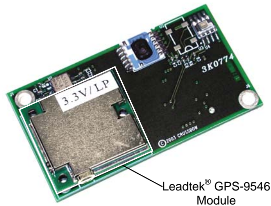
Figure 4-1. Photo of MTS420. The MTS400 does not have the GPS module (highlighted by the box).
