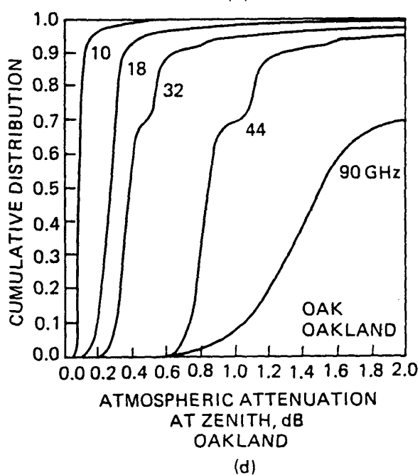
Exhibit 2.2.2.3-5 Cumulative Distributions of Zenith Cloud Attenuation at Four Locations, From the Slobin Cloud Model [Source: Slobin (1982)]
