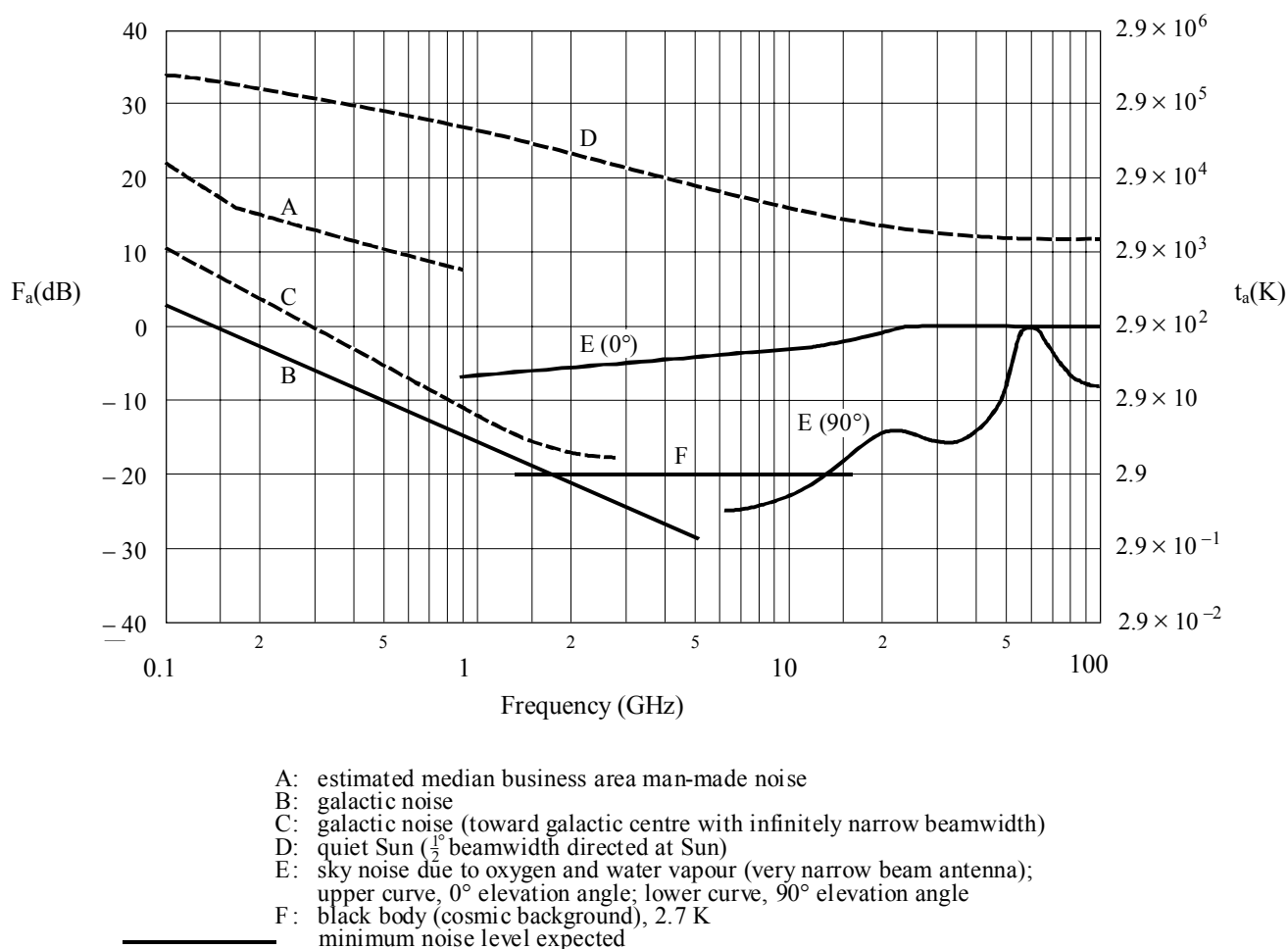
Exhibit 2.3.1-1 Noise Factor and Brightness Temperature from External Sources [Source: ITU-R PI.372-6 (1994)]
