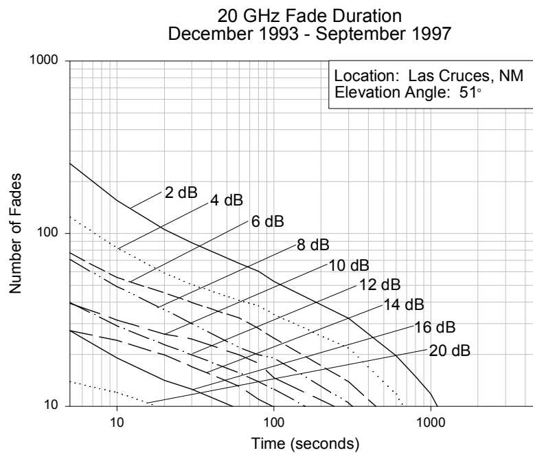
Exhibit 2.2.10.2-1: Fade Duration Calculated from New Mexico ACTS 20.2 GHz beacon data.
