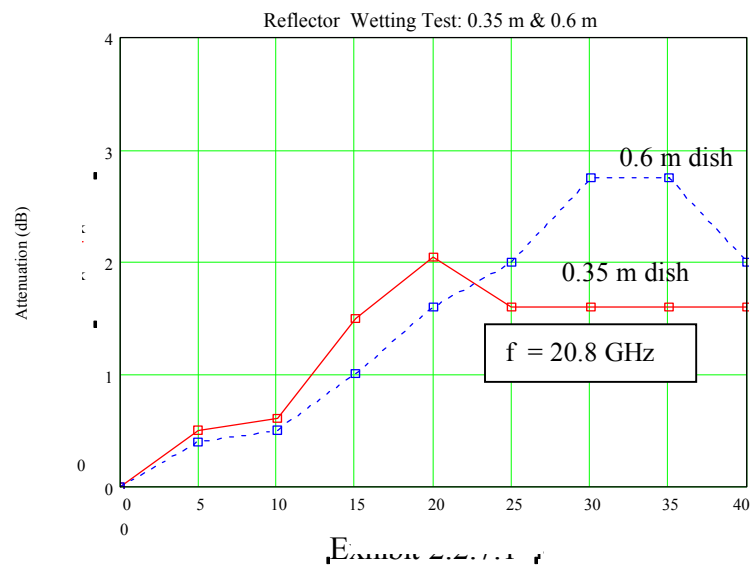
Dish Wetting Experiment for 0.35 m and 0.6 m parabolic antennas with F/D=0.6 (Acosta et al, 1997)
