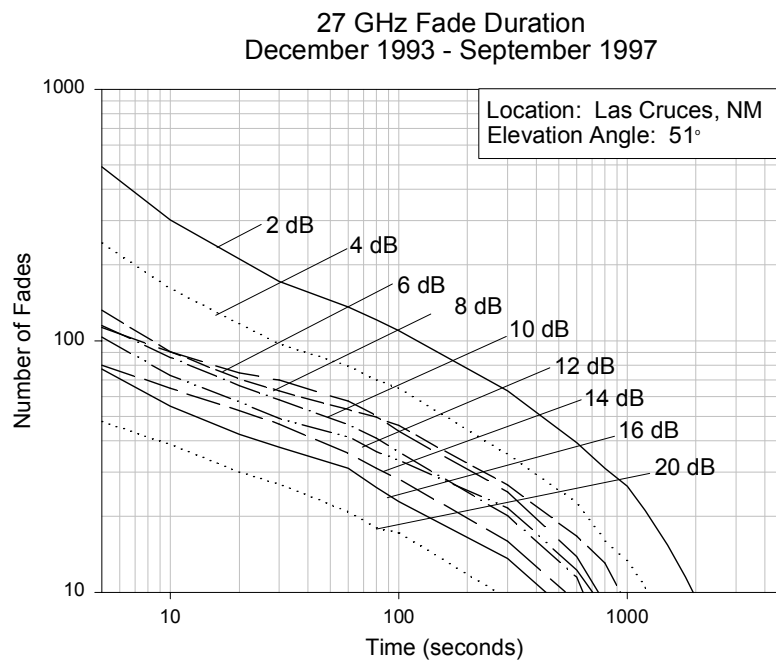
Exhibit 2.2.10.2-2: Fade Duration Calculated from New Mexico ACTS 27.5 GHz beacon data.
