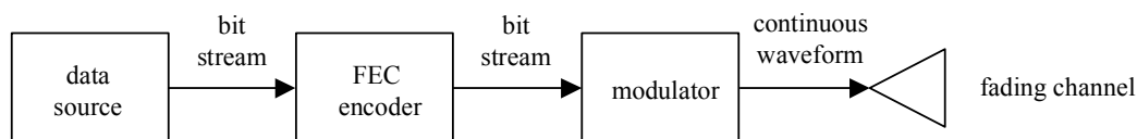
Transmitter
