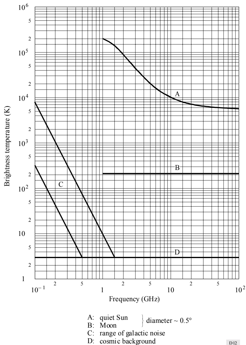
Exhibit 2.3.5-1 Extraterrestrial Noise Sources [Source: ITU-R Rec. PI.372-6 (1994)]
