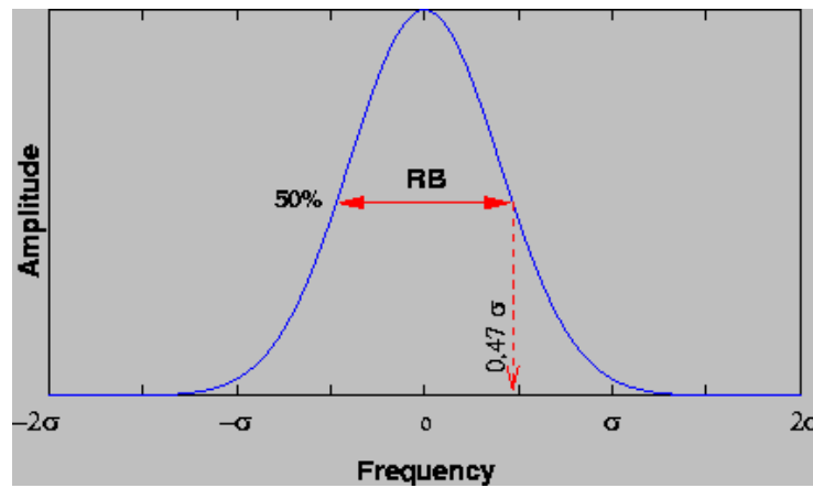
Figure 1: The Resolution Bandwidth ( RB ) is defined as the width at which the filter response falls to 50% of its maximum.
