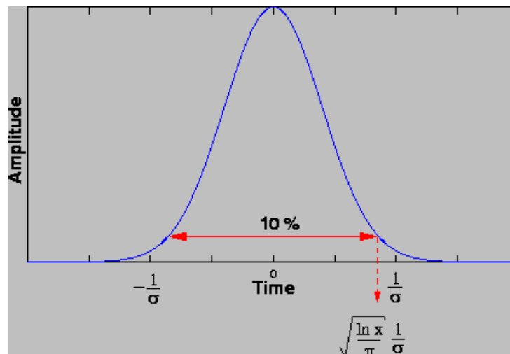
Figure 2: In this illustration, the time interval shown is sufficient for the filter to rise from 0.1 of its maximum response, and then fall back to 0.1. (This corresponds to x = 10 on slide 16.)
