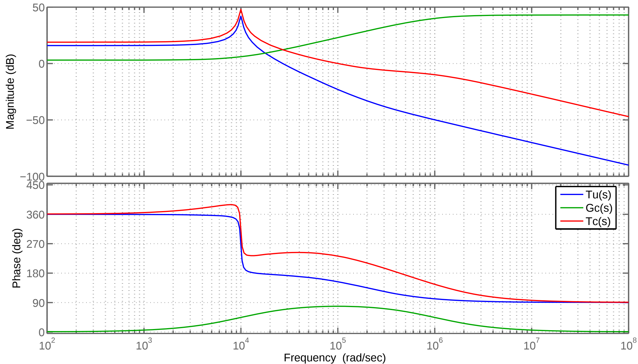
Bode Diagram
