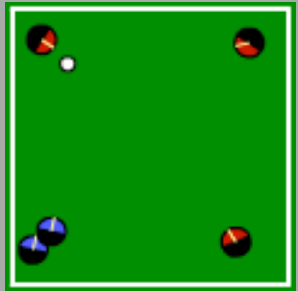
Learned
