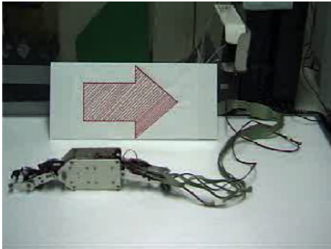
Backward
